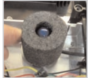
Photo Cell for Auto Dimming with Protective Shielding
