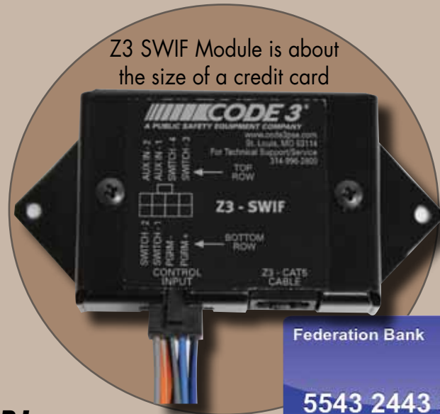
Ford P.I. Steering Wheel Remappable Switches
