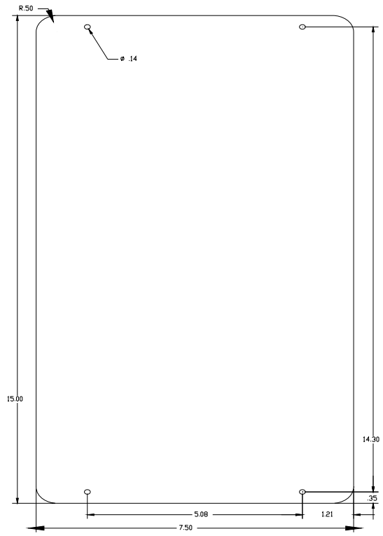
MOUNTING DIMENSIONS FOR 65STK3 4X6 LED PERIMETER TRIPLE STACK HOUSING
