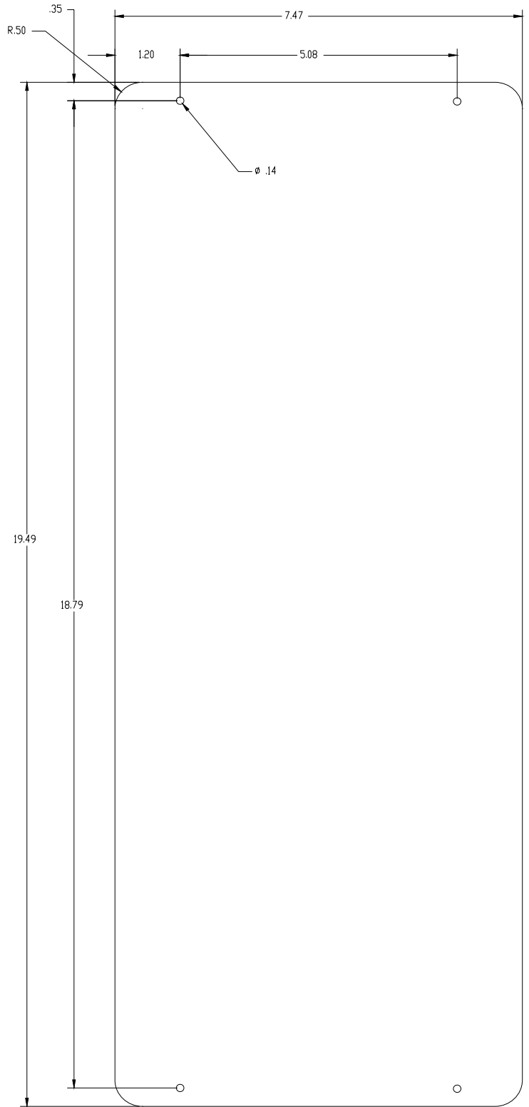
MOUNTING DIMENSIONS FOR 65STK4 4X6 LED PERIMETER QUAD STACK HOUSING
