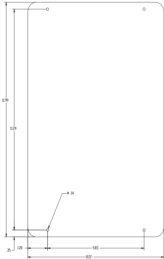
MOUNTING DIMENSIONS FOR 45STK3 3X7 LED PERIMETER TRIPLE STACK HOUSING
