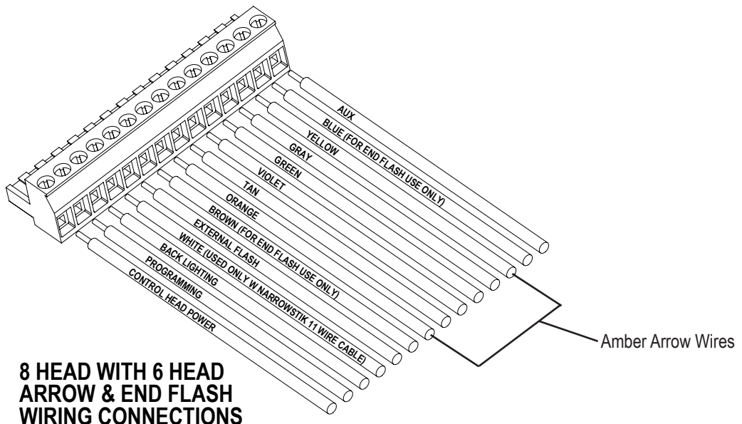
STANDARD 8 HEAD WIRING CONNECTIONS
